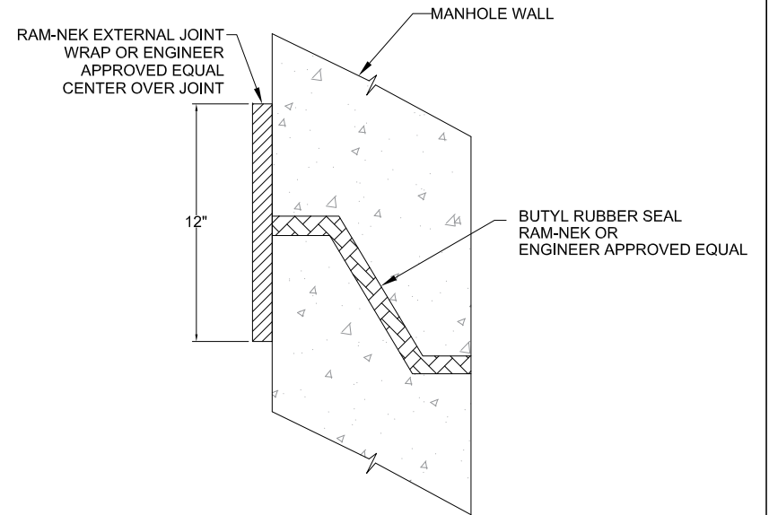
MANHOLE JOINT DETAIL
