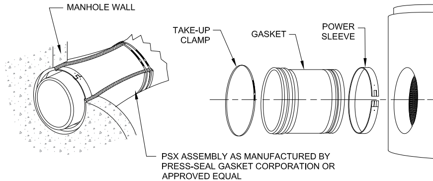
TYPICAL "BOOT" DETAIL
