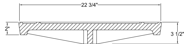
COVER SECTION VIEW N.T.S.
